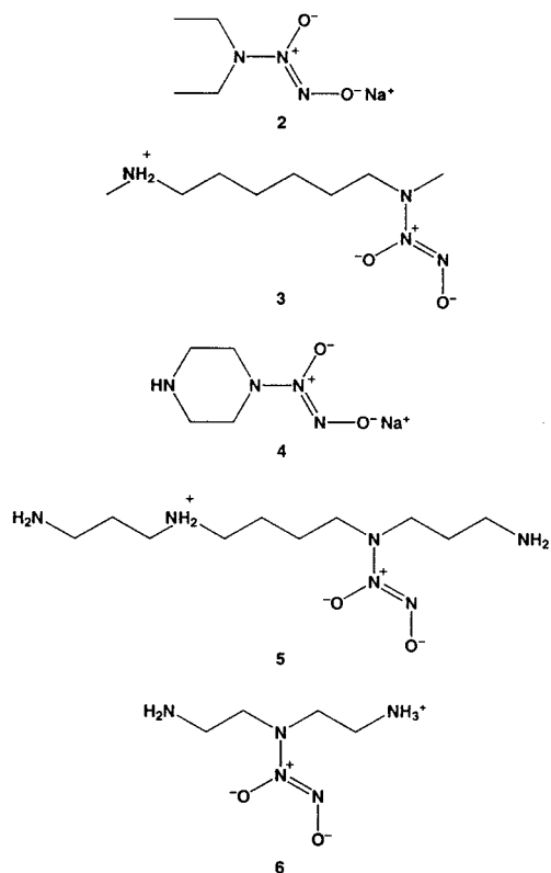
Figure 1. Structures of diazeniumdiolates included in this investigation.
